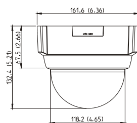
Hard ceiling mount
